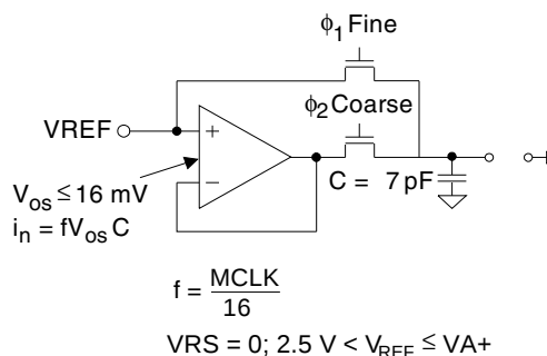
Figure 9. Input Reference Model when VRS = 0
