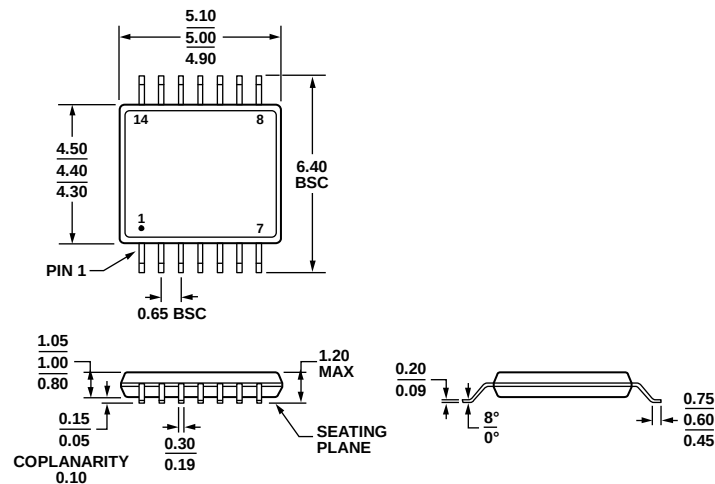
COMPLIANT TO JEDEC STANDARDS MO-153-AB-1
