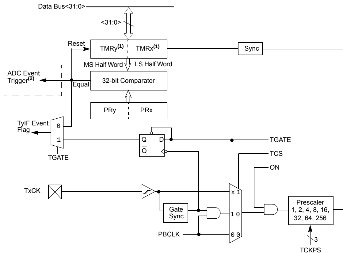
FIGURE 13-2: TIMER2/3, 4/5 BLOCK DIAGRAM (32-BIT) (1)
