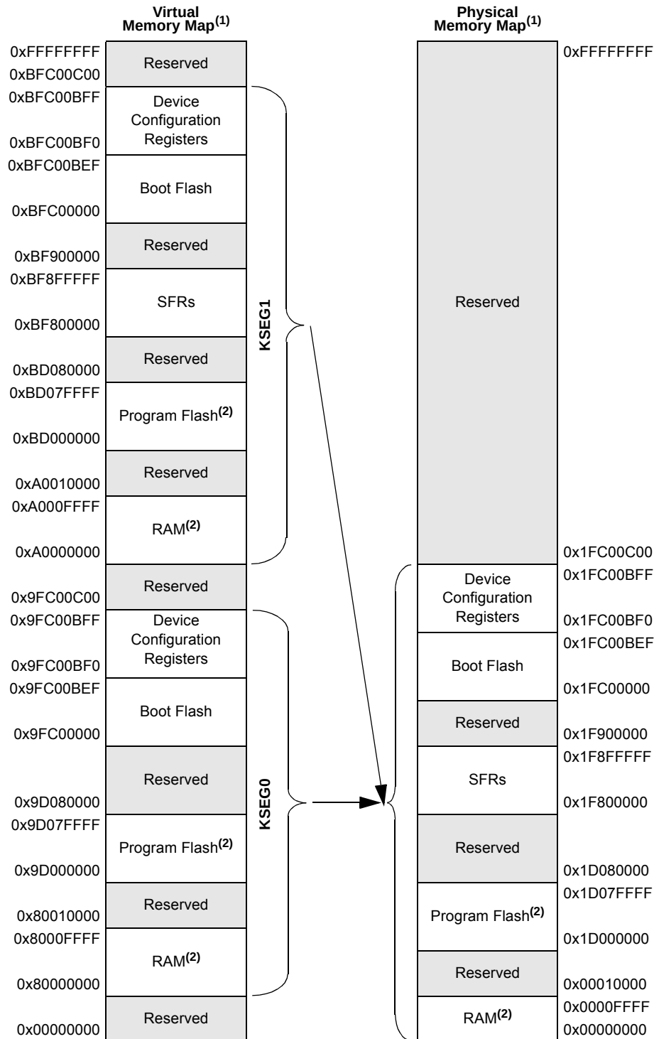
FIGURE 4-4: MEMORY MAP FOR DEVICES WITH 512 KB OF PROGRAM MEMORY + 64 KB RAM
