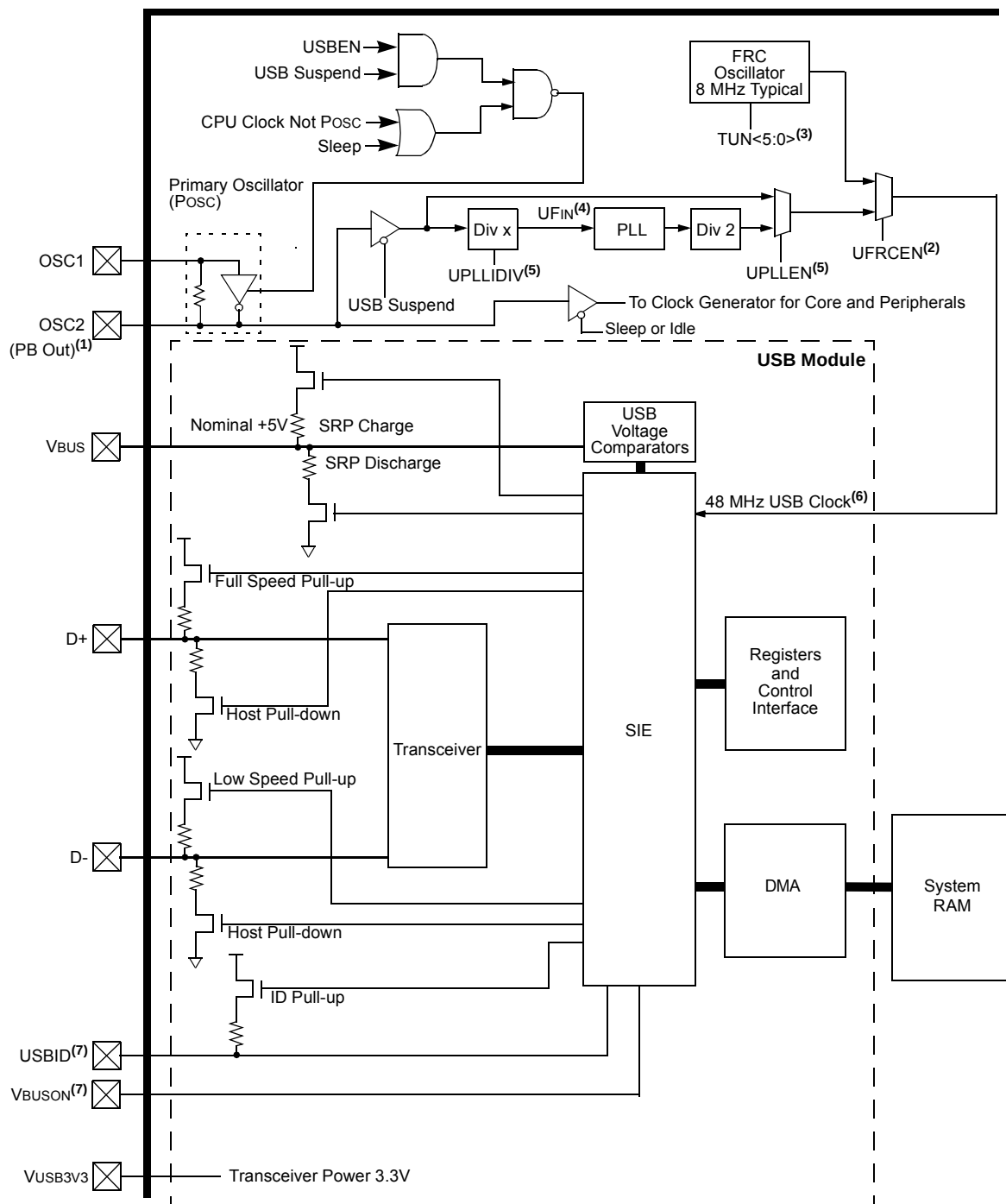
FIGURE 10-1: PIC32MX1XX/2XX/5XX USB INTERFACE DIAGRAM
