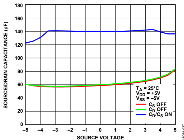
Figure 27. Source/Drain Capacitance vs. Source Voltage ( V_S )
