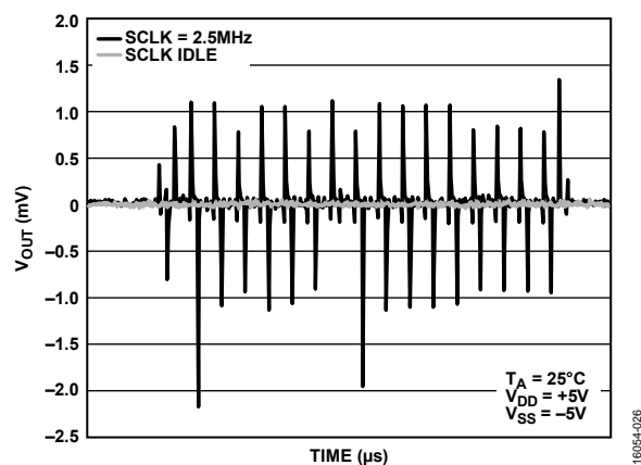
Figure 26. Digital Feedthrough
