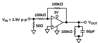
Figure 25. Output Swing, +V_S = +3V , G = -1
