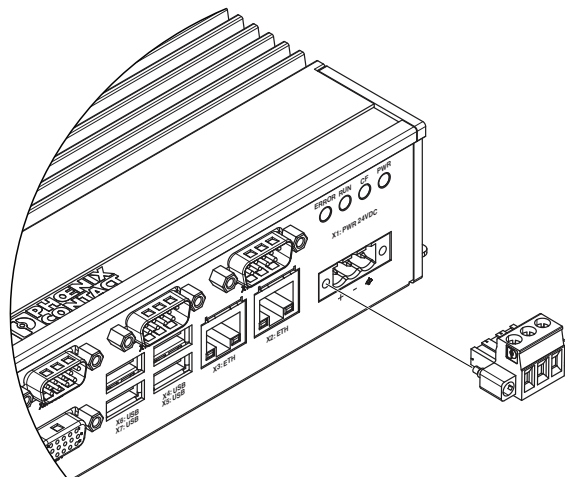
Figure 6 Power connector
