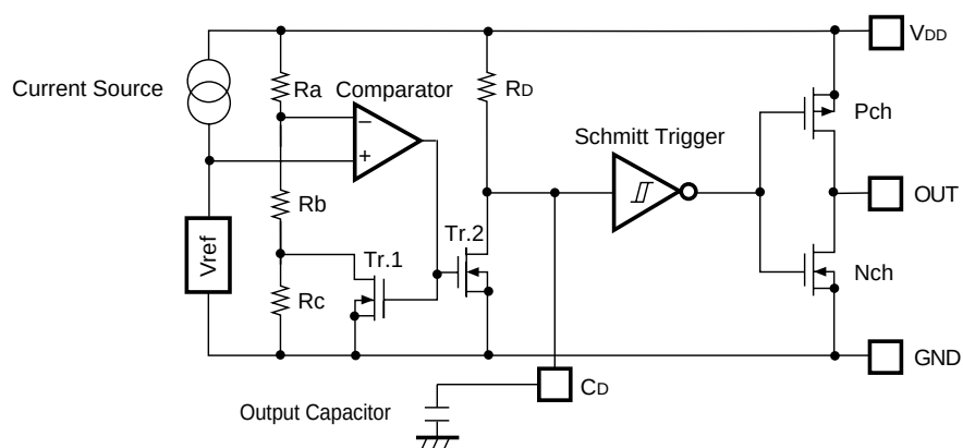
FIG. 1 Block Diagram
