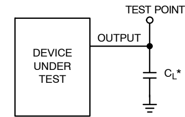
Figure 5. Test Circuit
