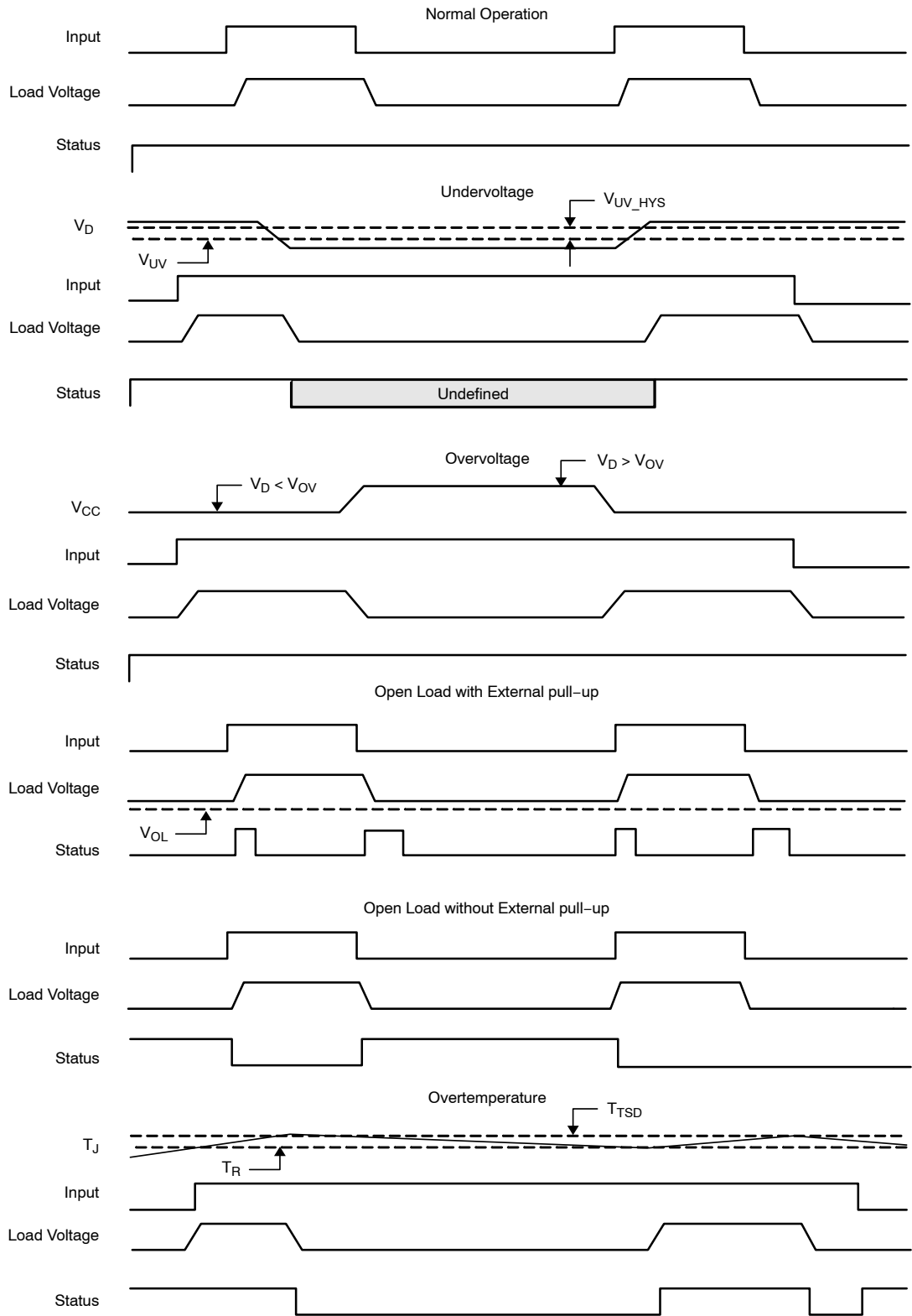
Figure 30. Waveforms
