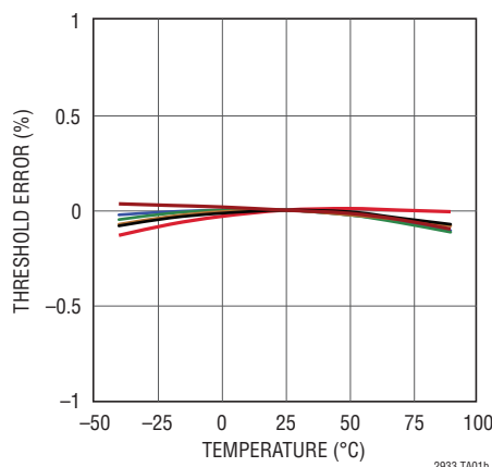
V1 to V6 Threshold Error vs Temperature
