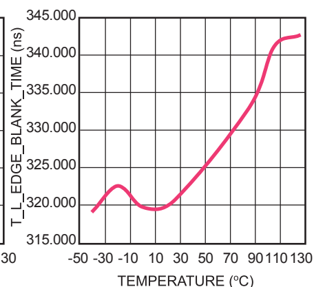
Leading Edge Blanking Time vs. Temperature
