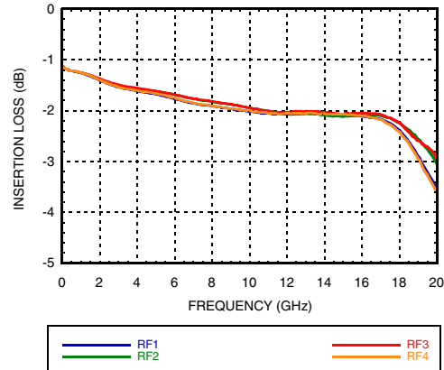
Insertion Loss over RF Ports
