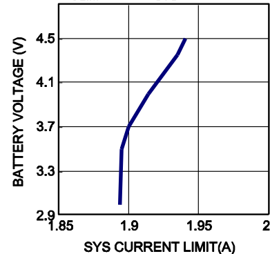
Programmable Output Currentlimit vs. Battery R_{OLIM}=59k\Omega , V_{SYS}=5V
