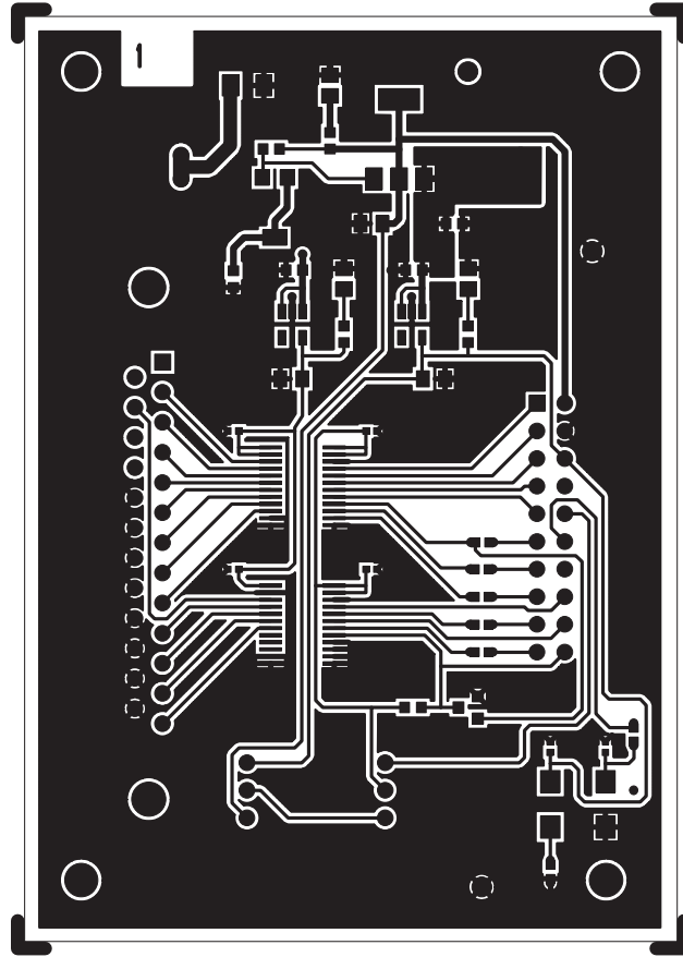
Figure 6-3. Layer 1 - Components Layer
