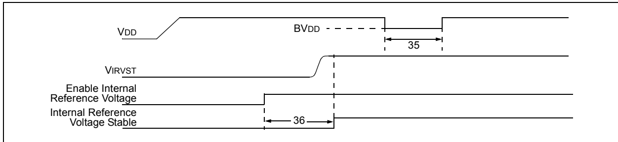
FIGURE 23-9: BROWN-OUT RESET TIMING
