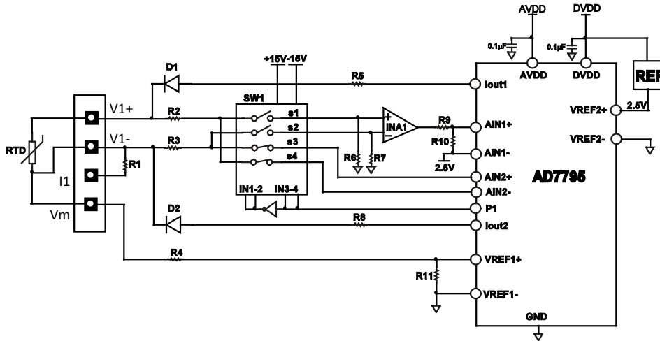
Figure 14. Ch2 Simplified RTD Input diagram
