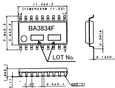
SOP18 (Unit: mm)
