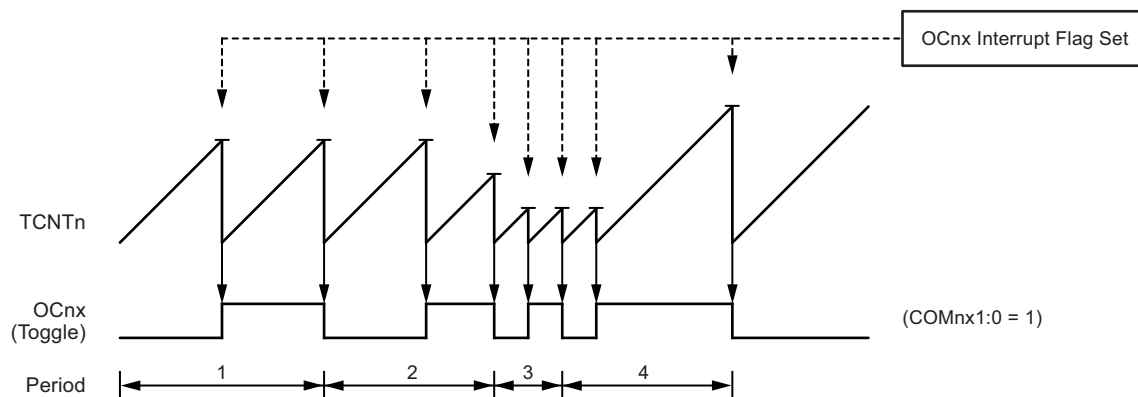
Figure 18-5. CTC Mode, Timing Diagram
