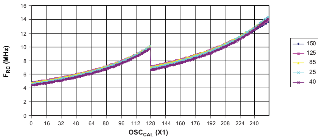
Figure 30-25. Calibrated 8MHz RC Oscillator Frequency versus OSCAL Value
