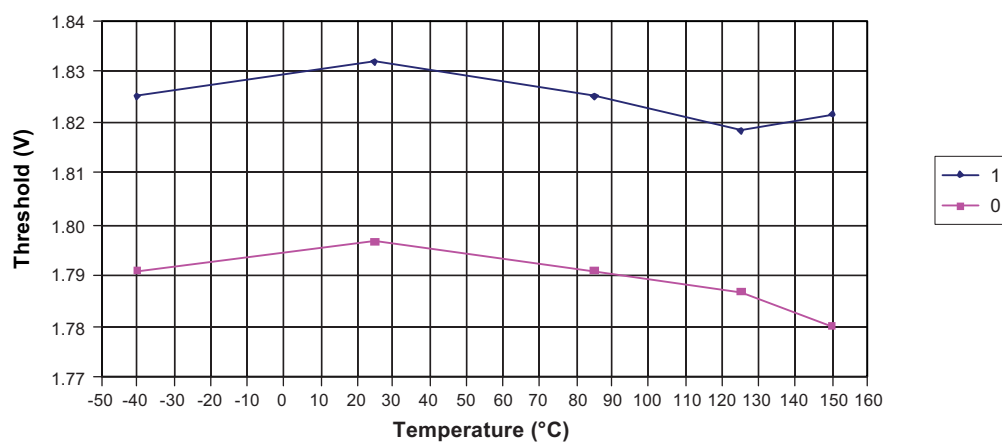
Figure 30-69. BOD Thresholds versus Temperature (BODLEVEL is 1.8V)
