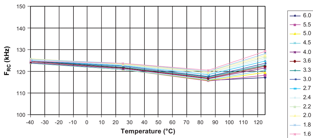
Figure 30-21. Watchdog Oscillator Frequency versus Temperature
