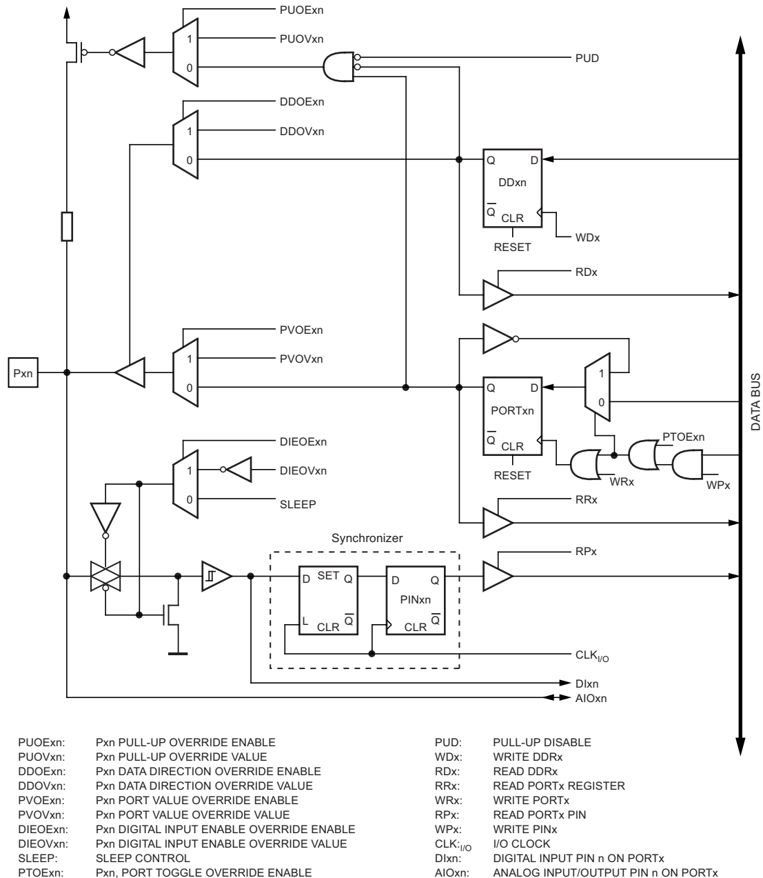
Figure 14-5. Alternate Port Functions (1)
