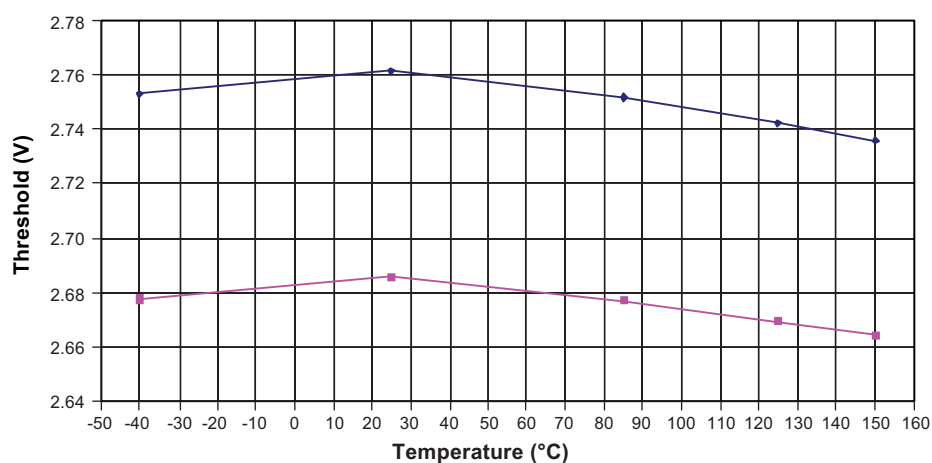
Figure 30-70. BOD Thresholds versus Temperature (BODLEVEL is 2.7V)
