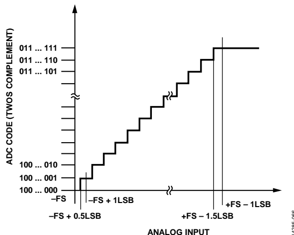
Figure 56. ADC Ideal Transfer Functions ( FS is Full Scale)
