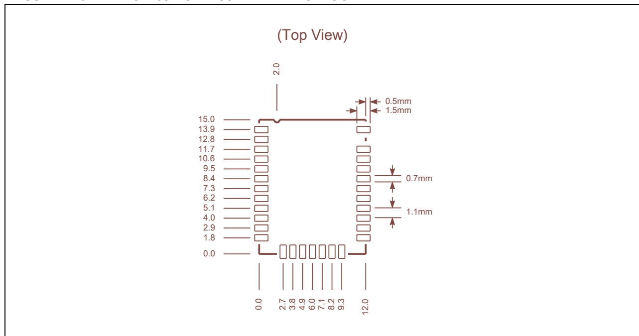
FIGURE 1-10: BM77SPP03MC2 RECOMMEDED PCB FOOTPRINT
