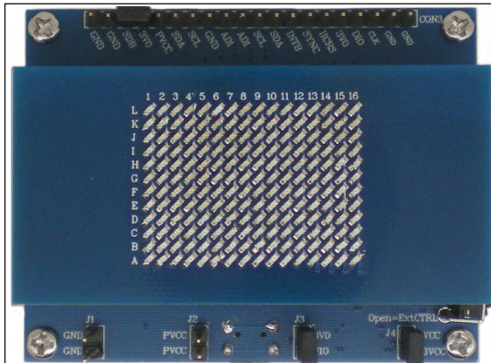
Figure 1: Photo of IS31FL3733 Evaluation Board
