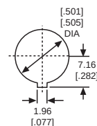
MOUNTING HOLE
