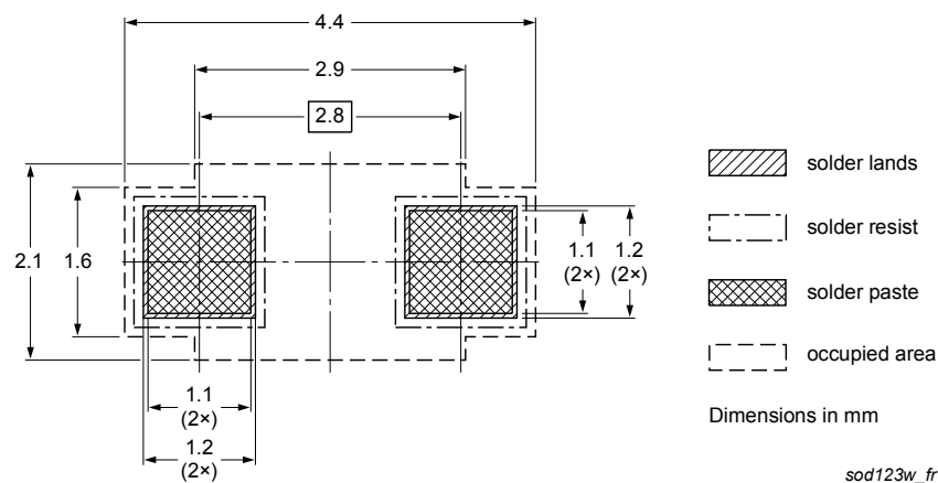
Fig. 19. Reflow soldering footprint for SOD123W
