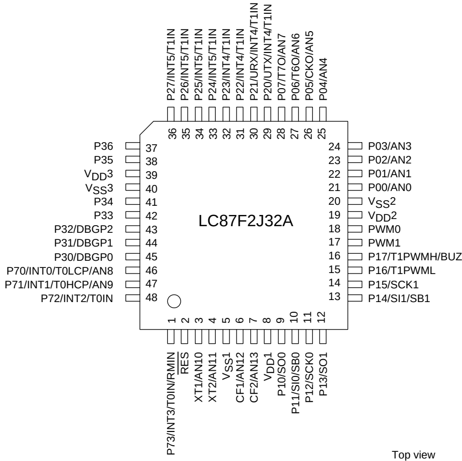
Top view
