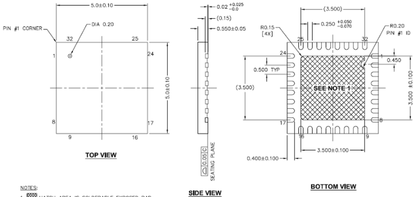
Figure 16. 32-Pin (5x5 mm) QFN
