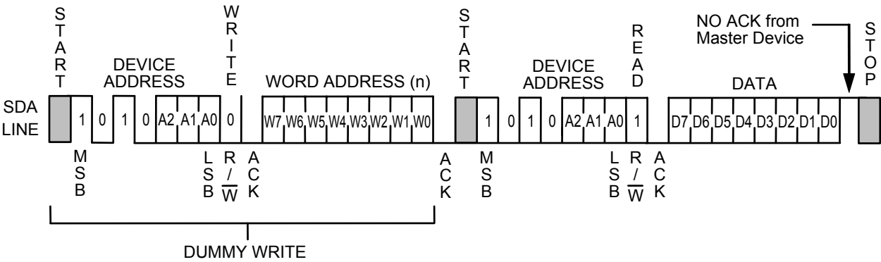
Figure 15 Random Read
