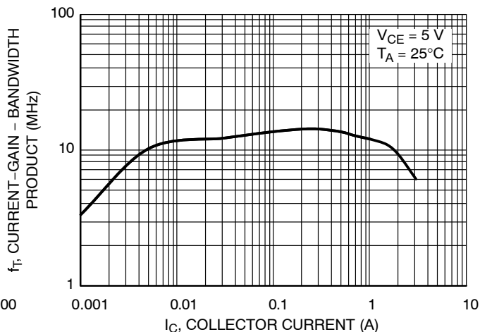
Figure 13. Current-Gain-Bandwidth Product
