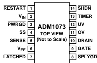
Figure 2. Pin Configuration
