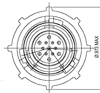
Free Style Plug with integral Backshell for Micro Band Strap and Heatshrink Boot Pin Contacts with Solder Bucket Termination Replace * with Orientation N or F
