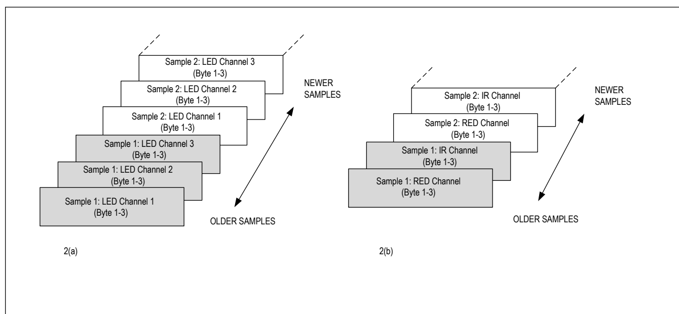
Figure 2.a and 2b. Graphical Representation of the FIFO Data Register. The left shows three LEDs in multi-LED mode, and the right shows IR and Red only in SpO 2 Mode.
