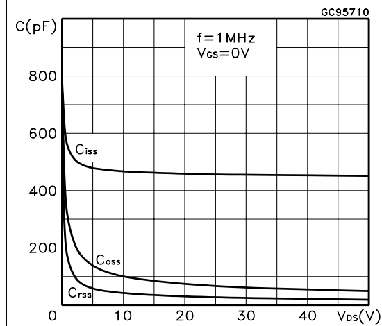
Figure 8: Capacitance variations
