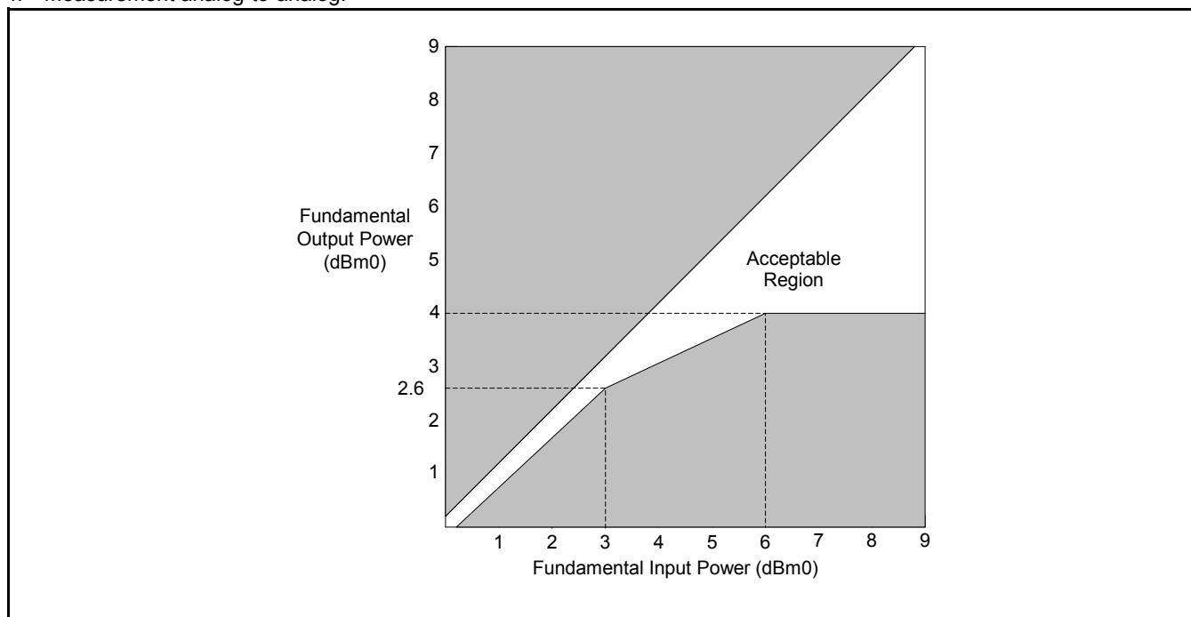
Figure 26 - Analog-to-Analog Overload Compression
