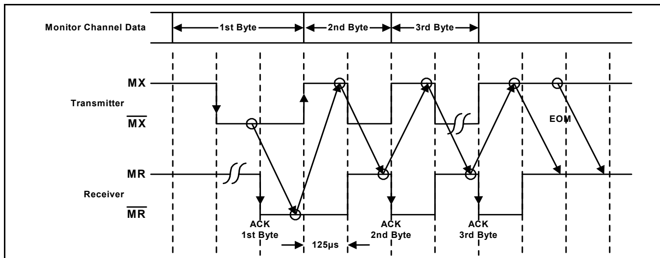
Figure 11 - Maximum Speed Monitor Handshake Timing
