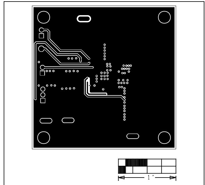
Figure 5. MAXM17503 EV Kit PCB Layout—PGND Layer 3
