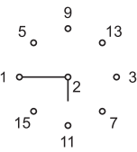
20 Rotary selector switching element 45° page 55
