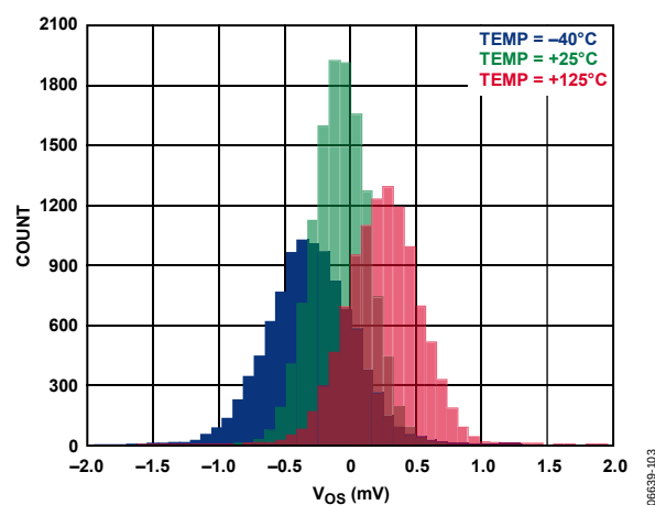
Figure 24. Offset Distribution ( V_{OS} ), V_{CM} = 6 V
