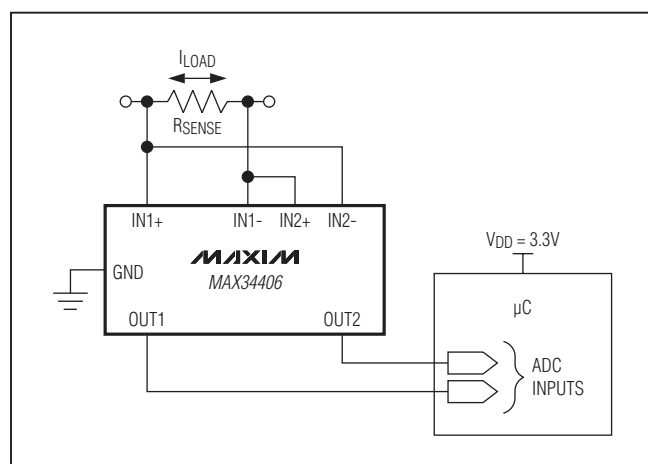
Figure 3. Bidirectional Application
