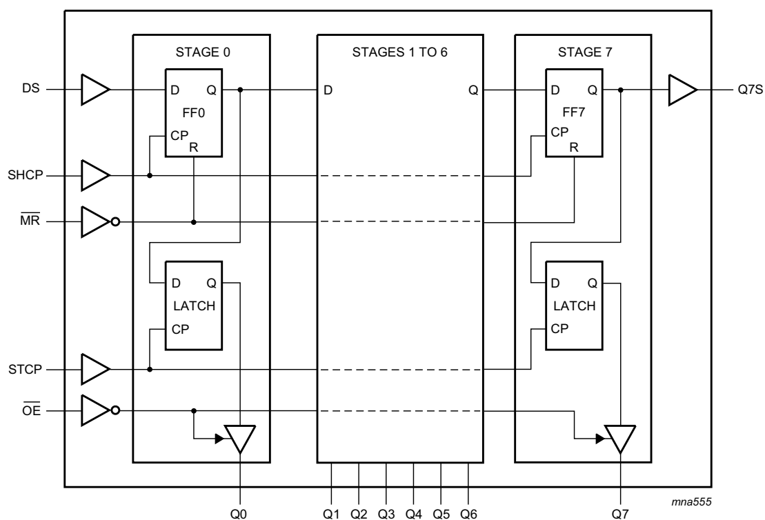
Fig 4. Logic diagram
