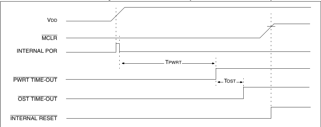
FIGURE 3-5: TIME-OUT SEQUENCE ON POWER-UP ( \overline{\text{MCLR}} NOT TIED TO \text{V}_{\text{DD}} ): CASE 2
