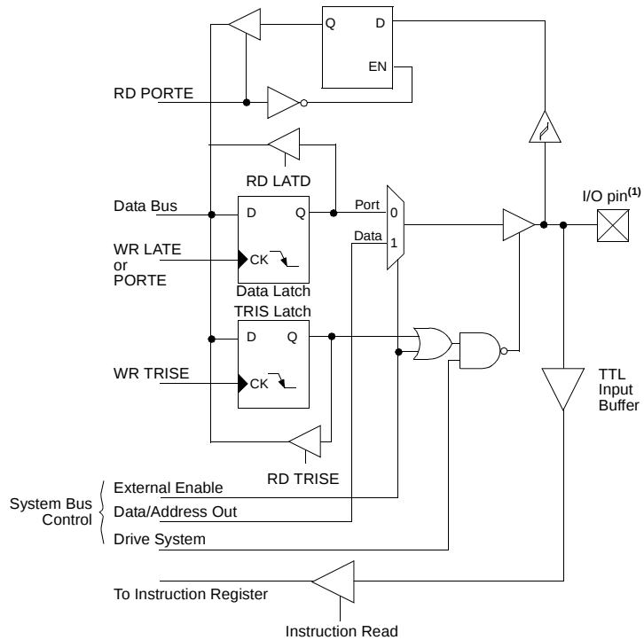
FIGURE 9-10: PORTE BLOCK DIAGRAM IN SYSTEM BUS MODE
