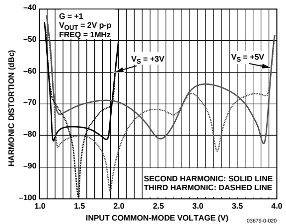
Figure 23. Harmonic Distortion vs. Input Common Mode Voltage
