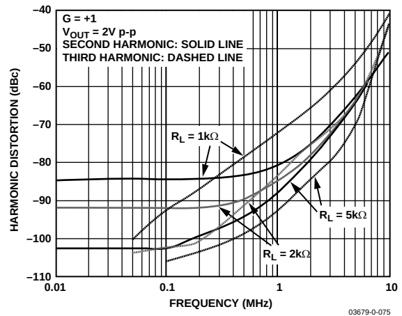
Figure 22. Harmonic Distortion vs. Frequency and Load
