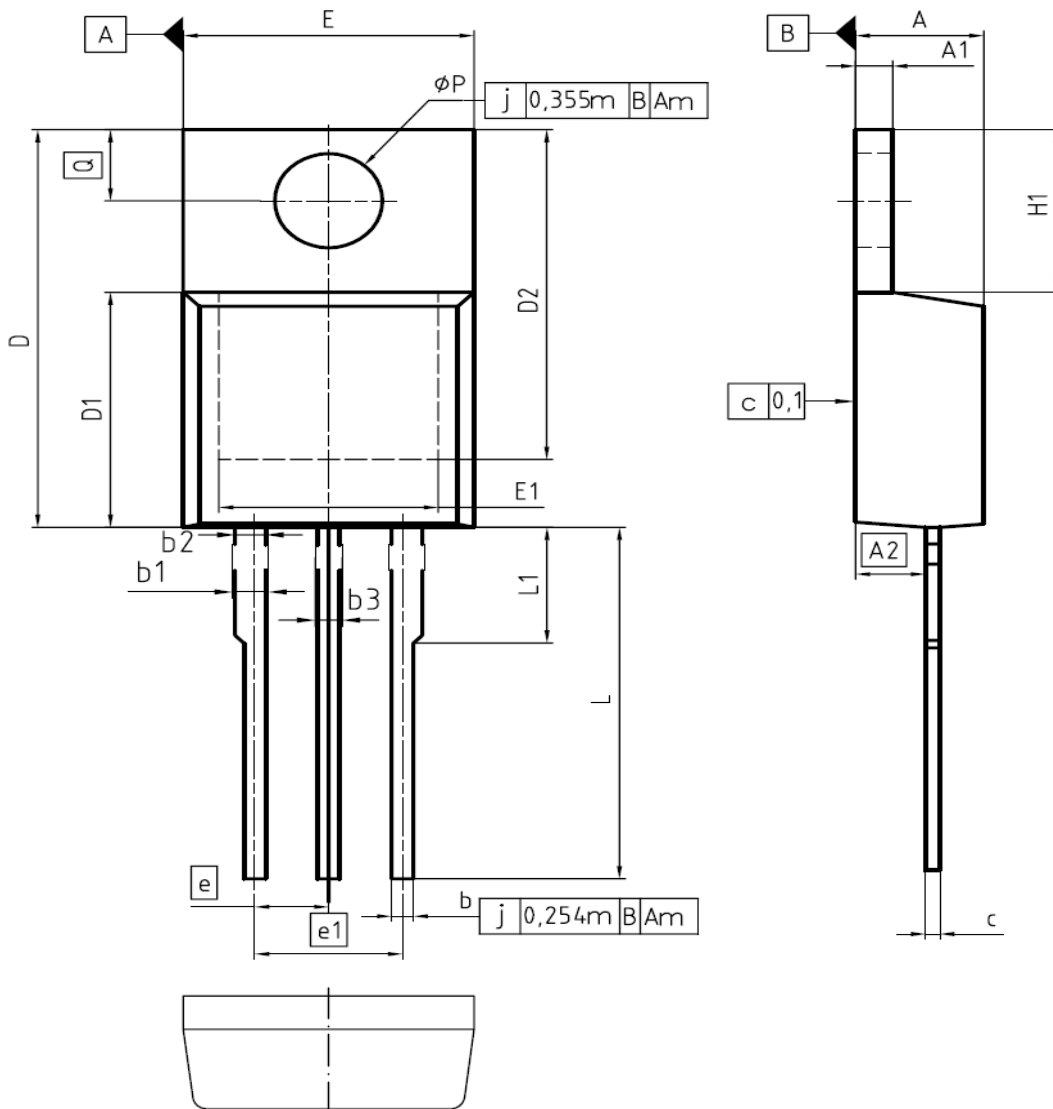
PG-TO-220-3-1
