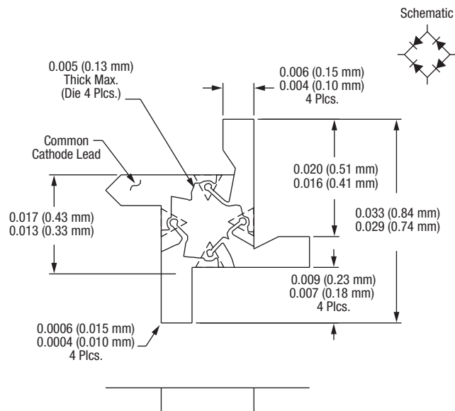
Figure 23. 488-004 Package Dimensions
