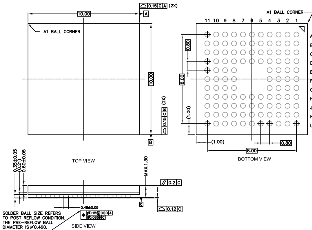
Figure 4.2. BGA112
