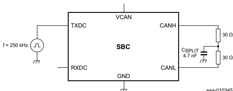
Fig 33. Test circuit for measuring transceiver driver symmetry
