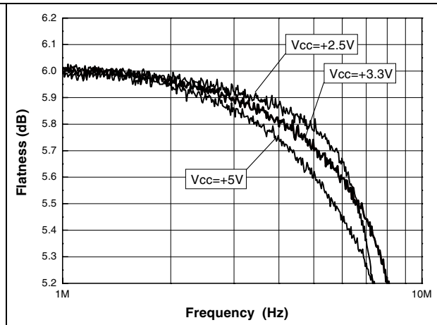
Figure 2. Gain flatness
