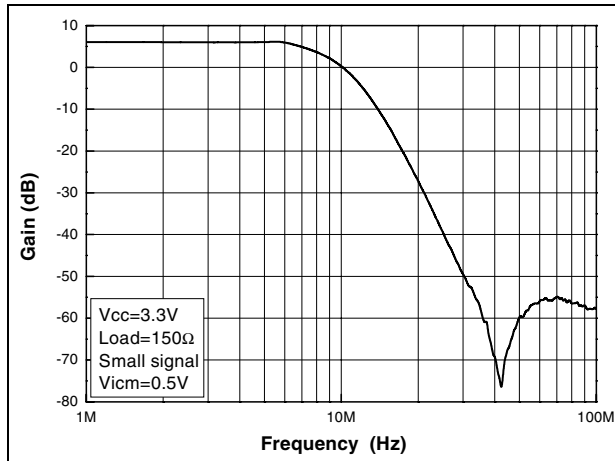
Figure 1. Frequency response
