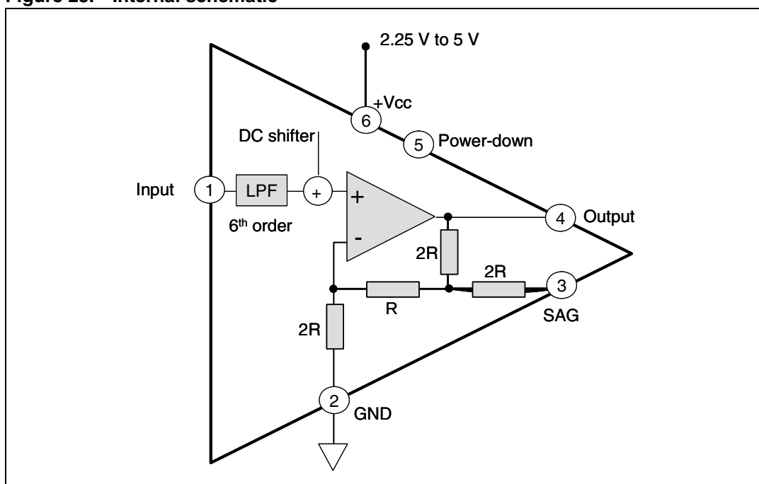
Figure 25. Internal schematic
