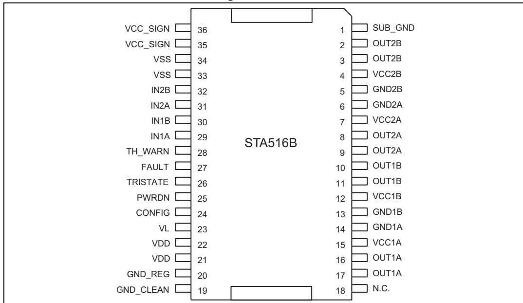
Figure 2. Pin out
